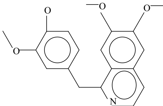
Fig 2.79: Structure of Papaverine
