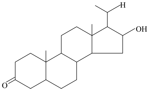
Fig 16.8: Structure of Guggulsterone
