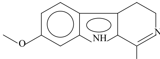
Fig 2.49 : Structure of Harmaline
