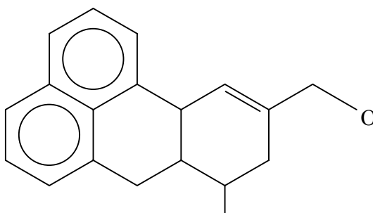
Fig 2.42 Structure of Elymoclavine
